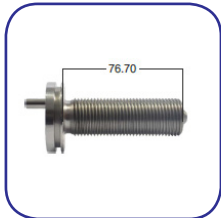
WABPAN192201 Caliper Bolt
